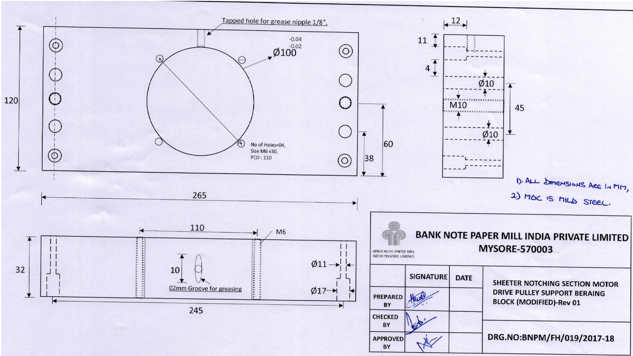
DRAWING:- BEARING BLOCK (BNPM/FH/019/2017-18)
